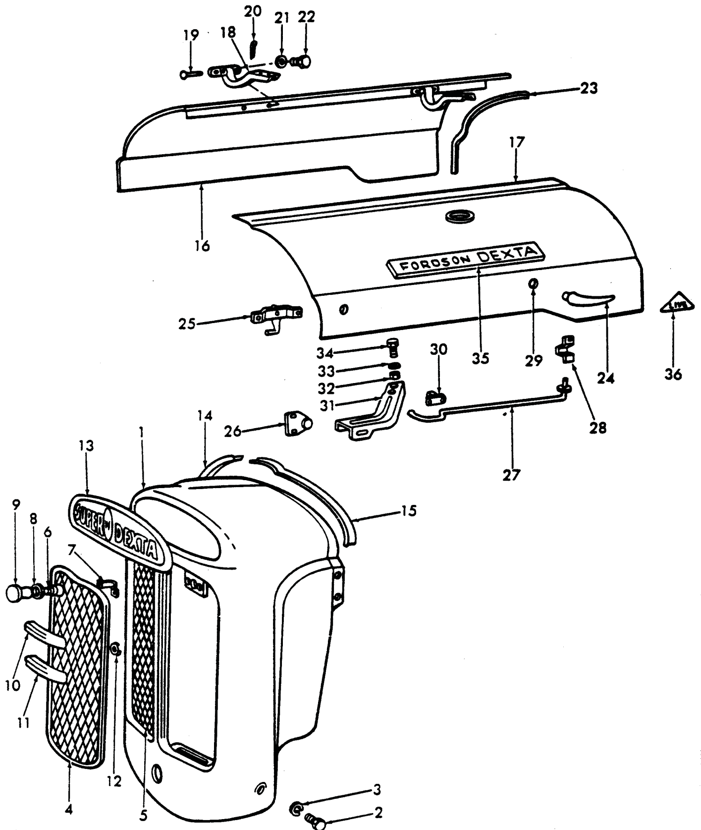
Fig. 56 Engine Hood, Grille & Related Parts
