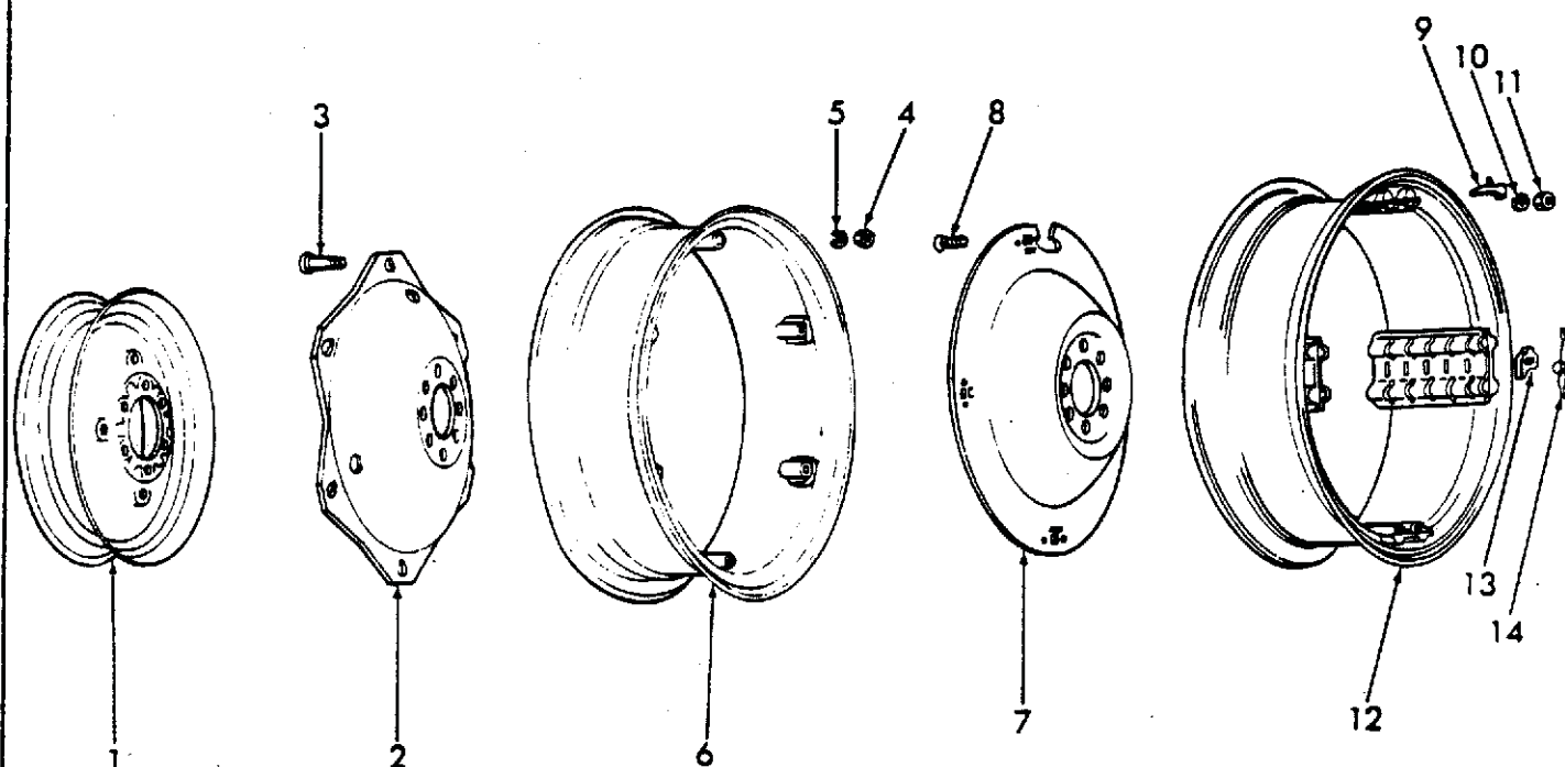
Fig. 1 Wheels & Weights
