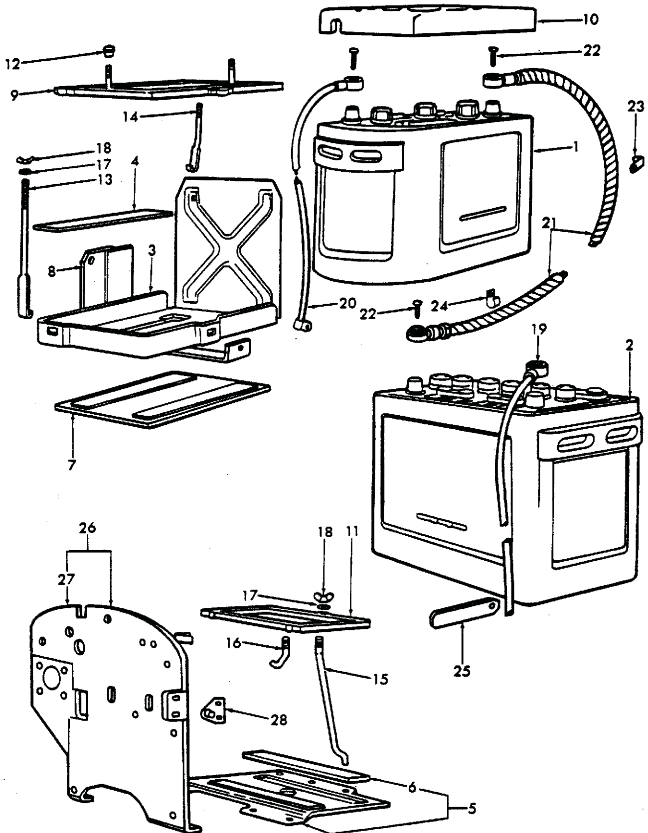
Fig. 48 Battery & Tray
