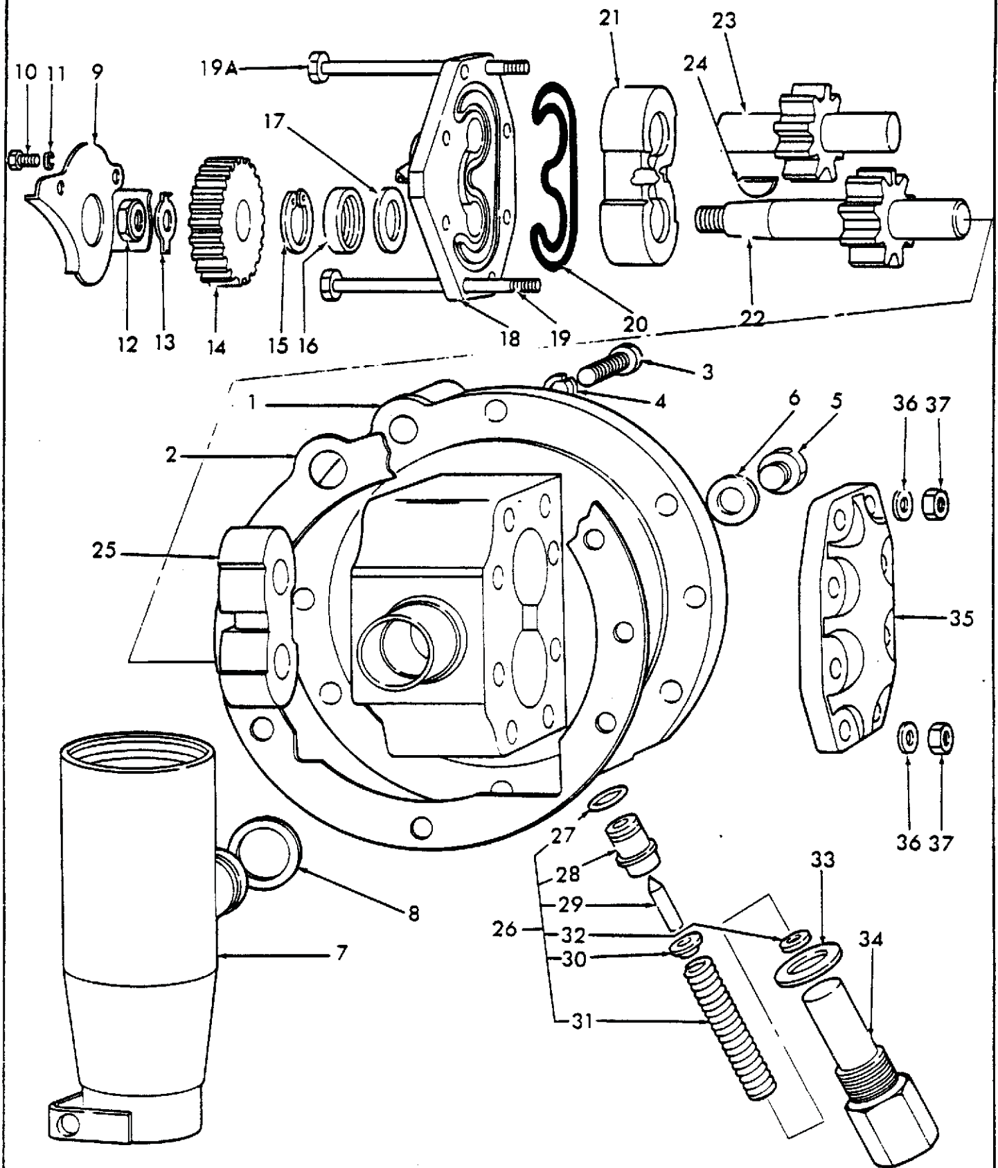
Fig. 13 Hyd. Power Lift Pump
