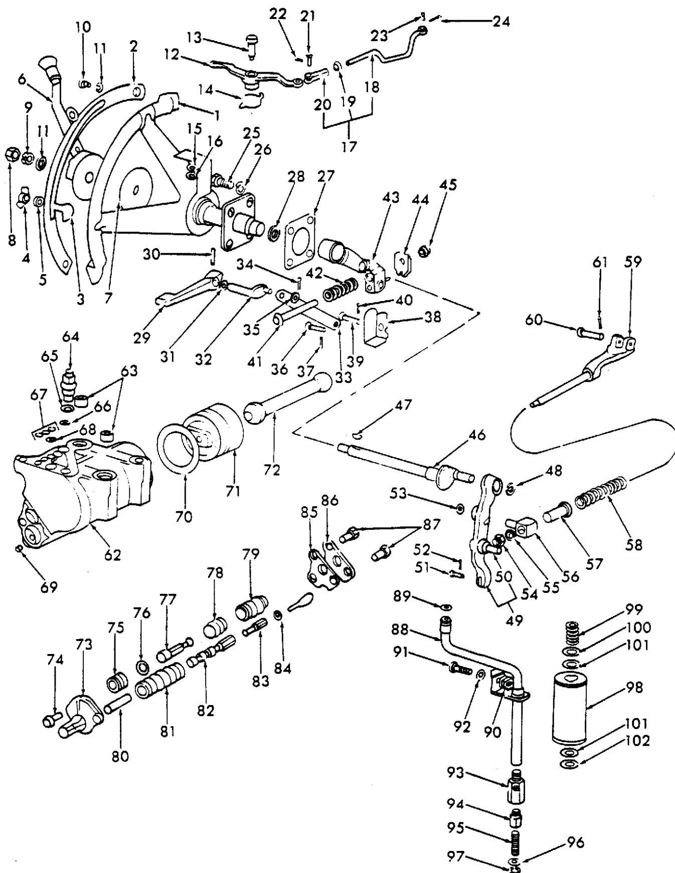
Fig. 11 Hyd. Lift Ram Cyl. & Related Parts
