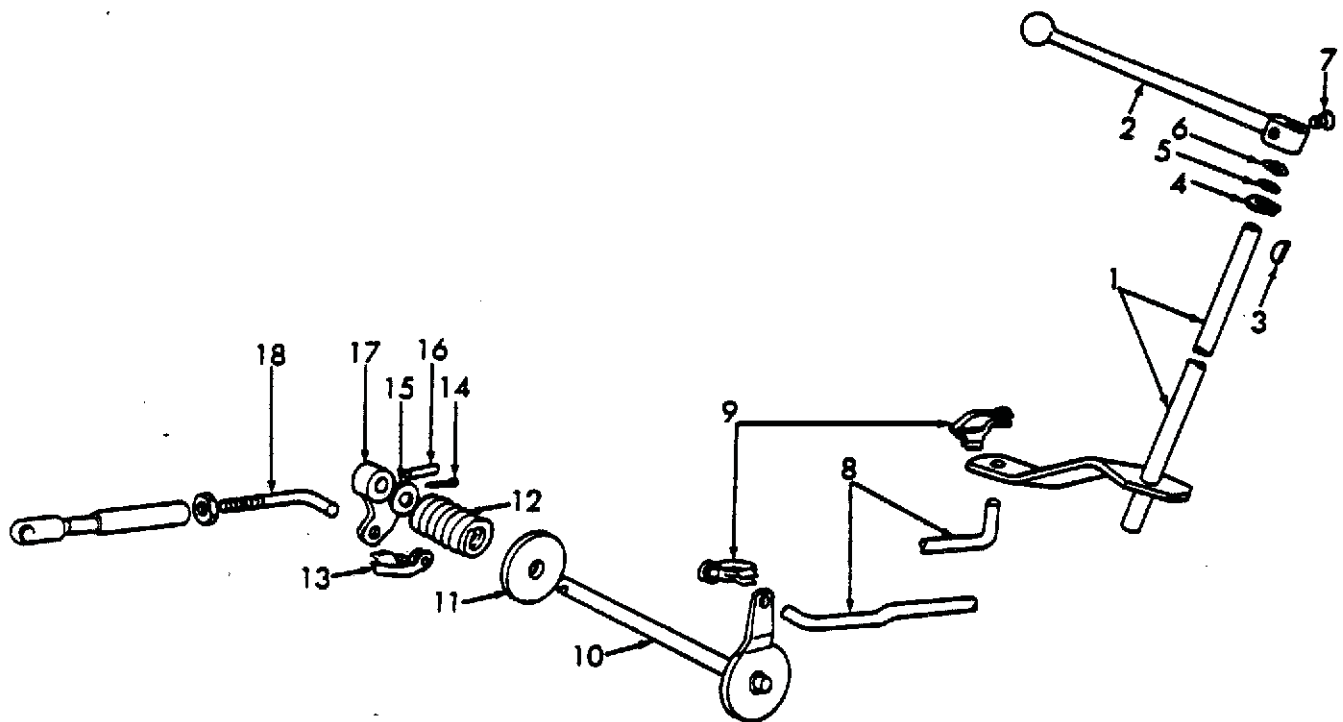
THROTTLE CONTROL PNEUMATIC GOVERNOR
