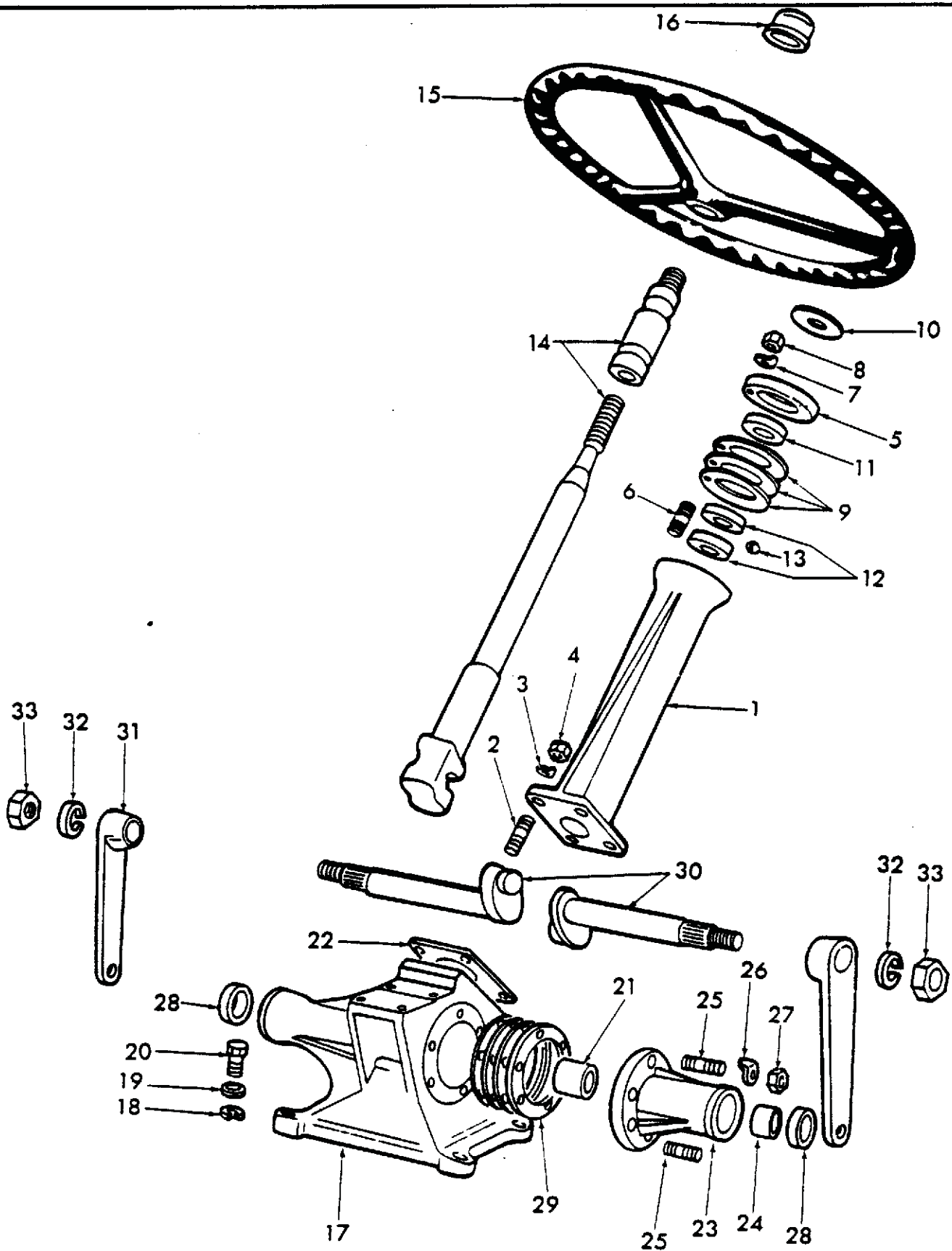
Fig. 6 Steering Gear
