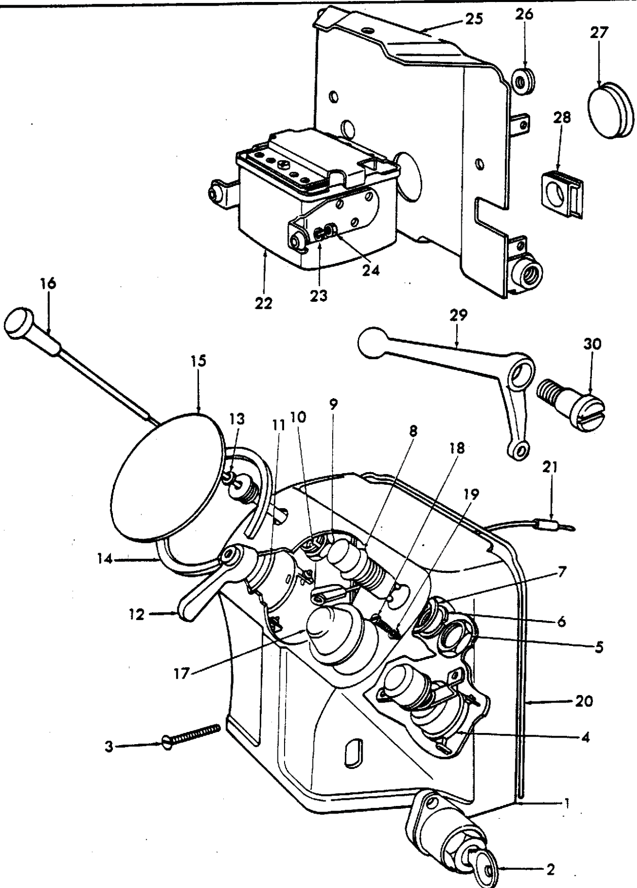
Fig. 52 Instrument Box
