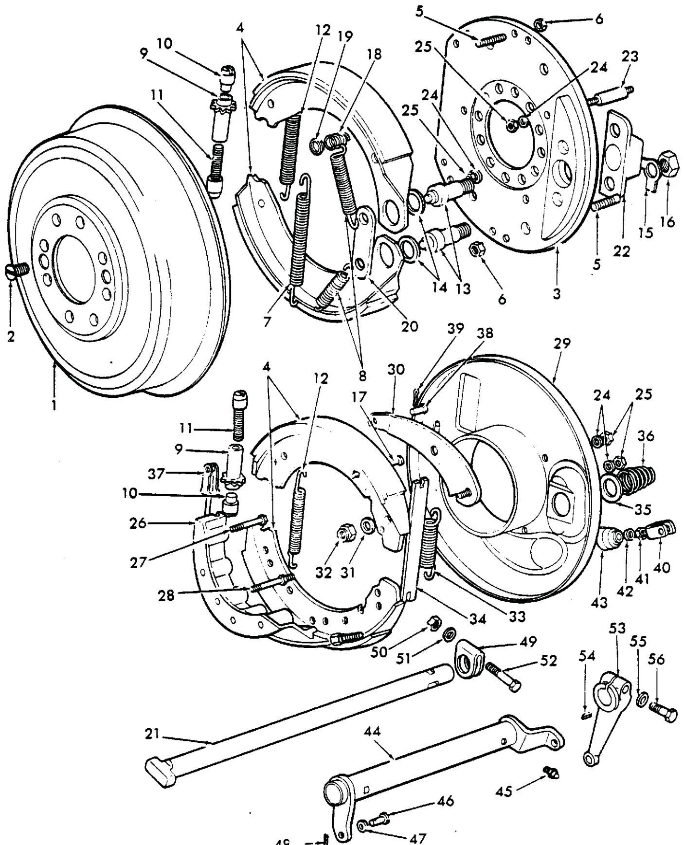
Fig. 3 Dual Rear Brakes
