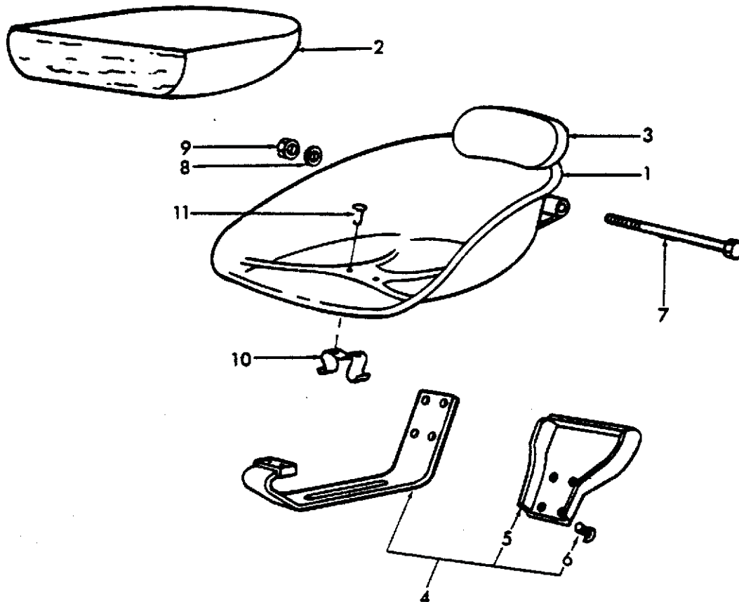
Fig. 54 Seat Assemblies
