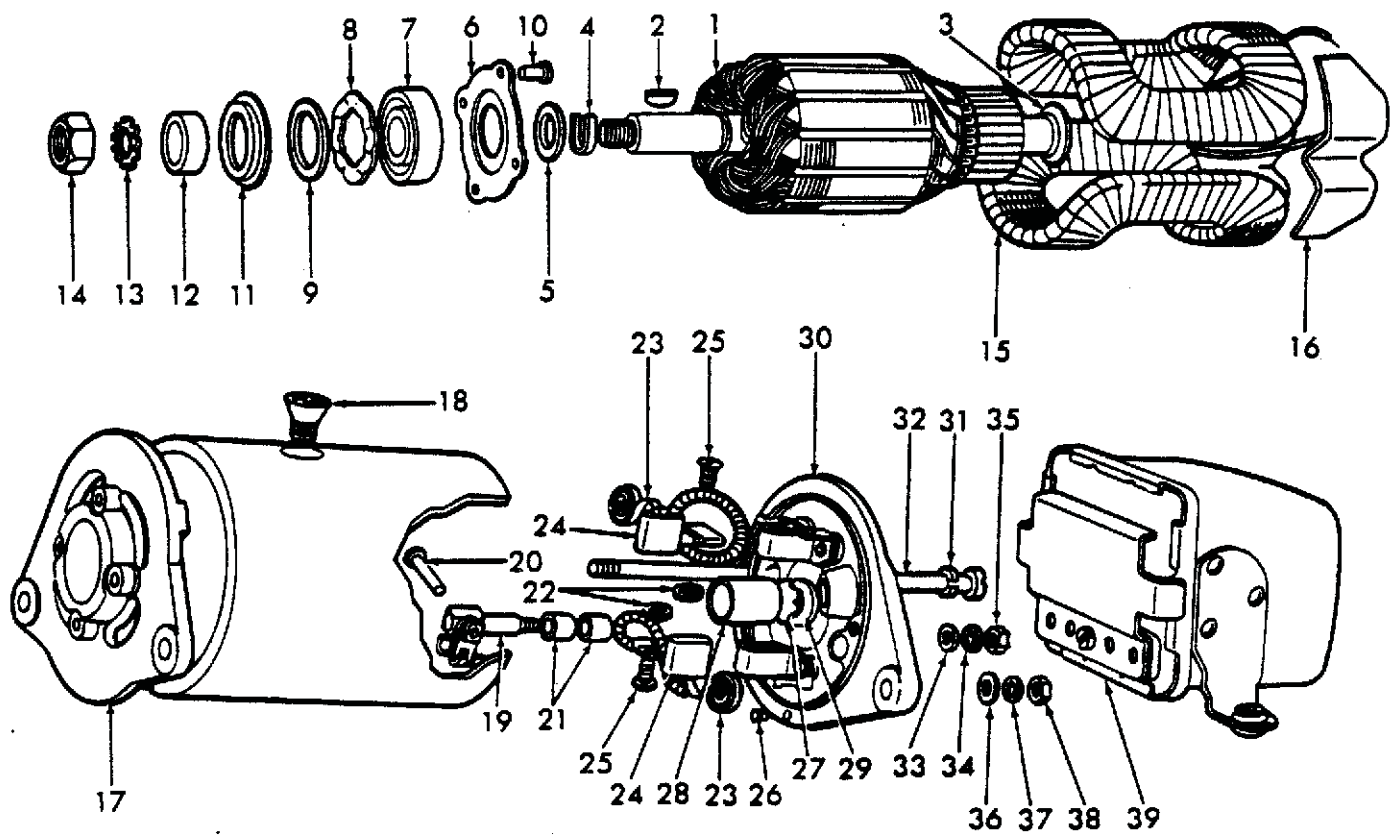
GENERATOR AND REGULATOR-57/10-62
