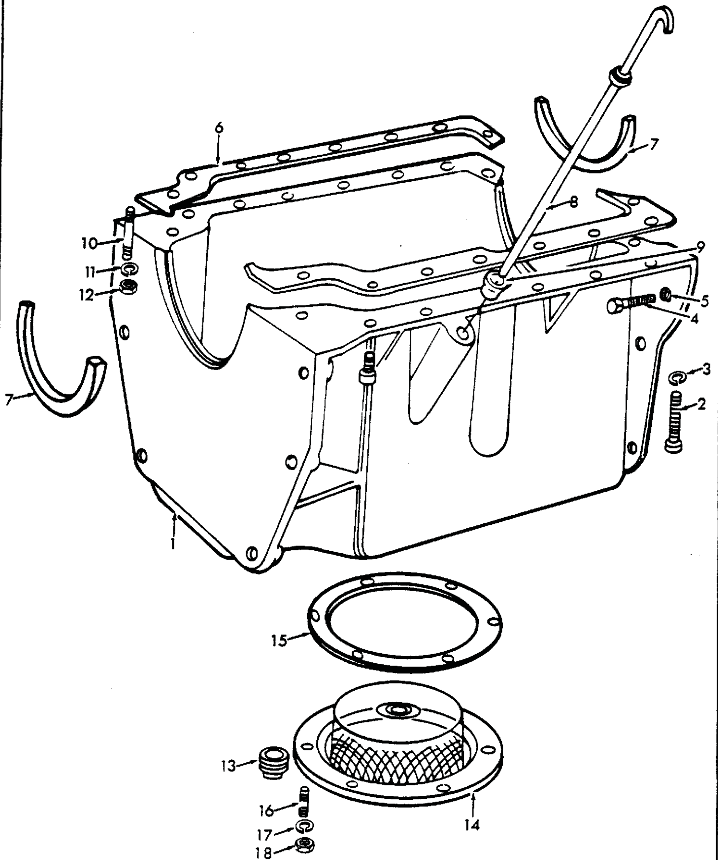
Fig. 23 Oil Pan & Related Parts
