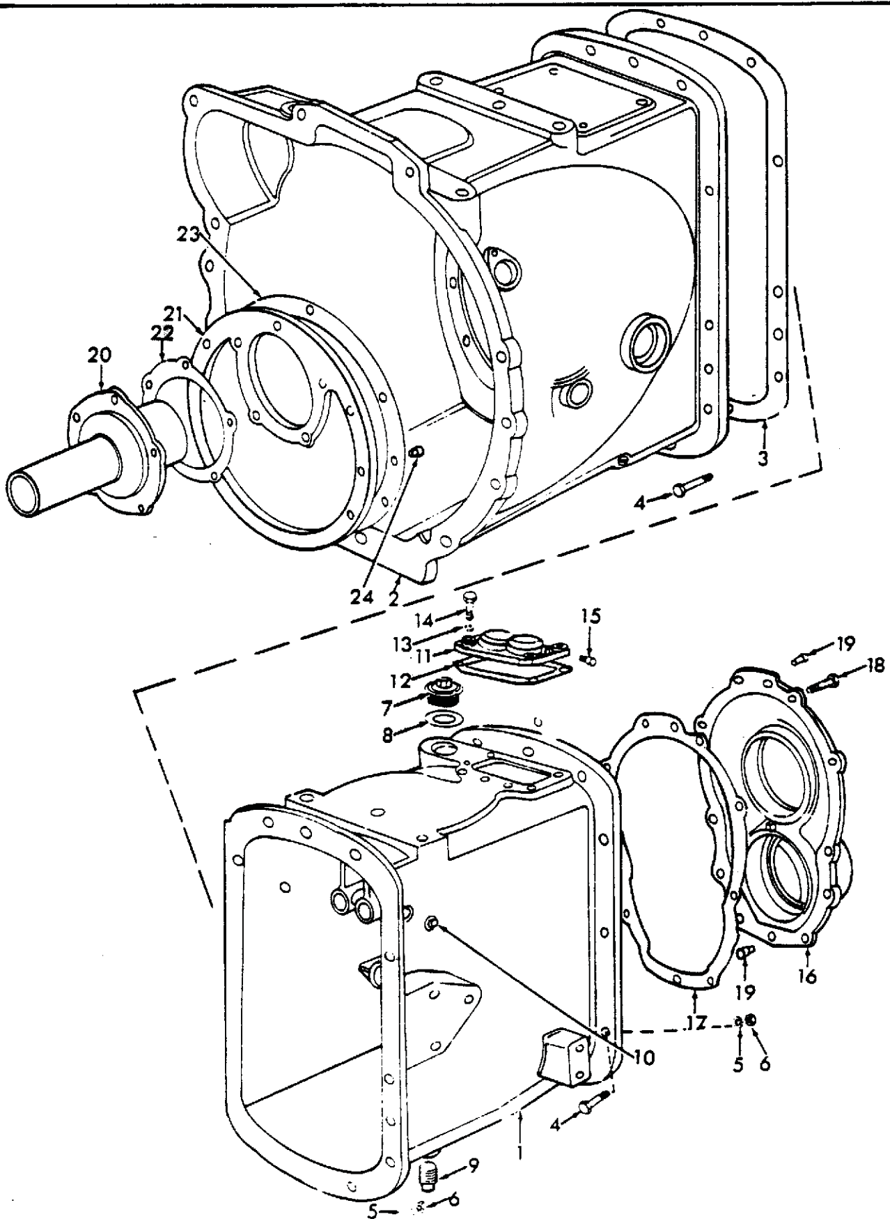
Fig. 27 Transmission & Clutch Housing
