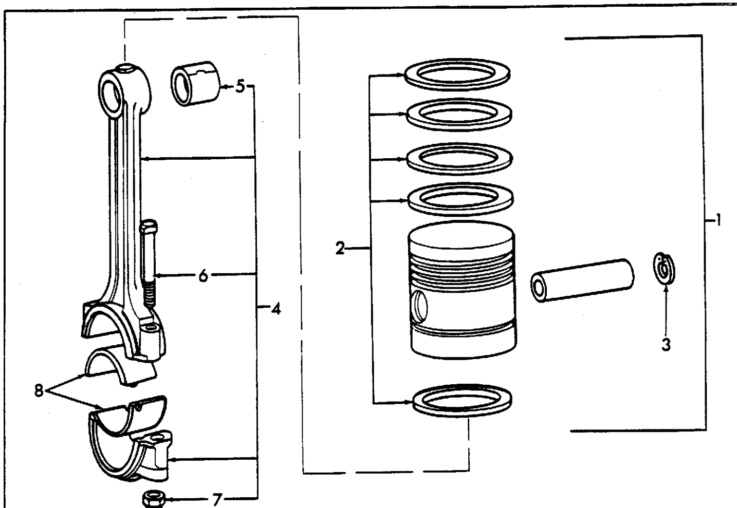
Fig. 22 Piston & Connecting Rods
