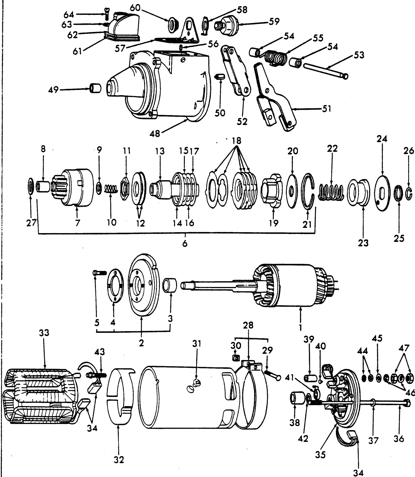
Fig. 49 Starting Motor & Related Parts
