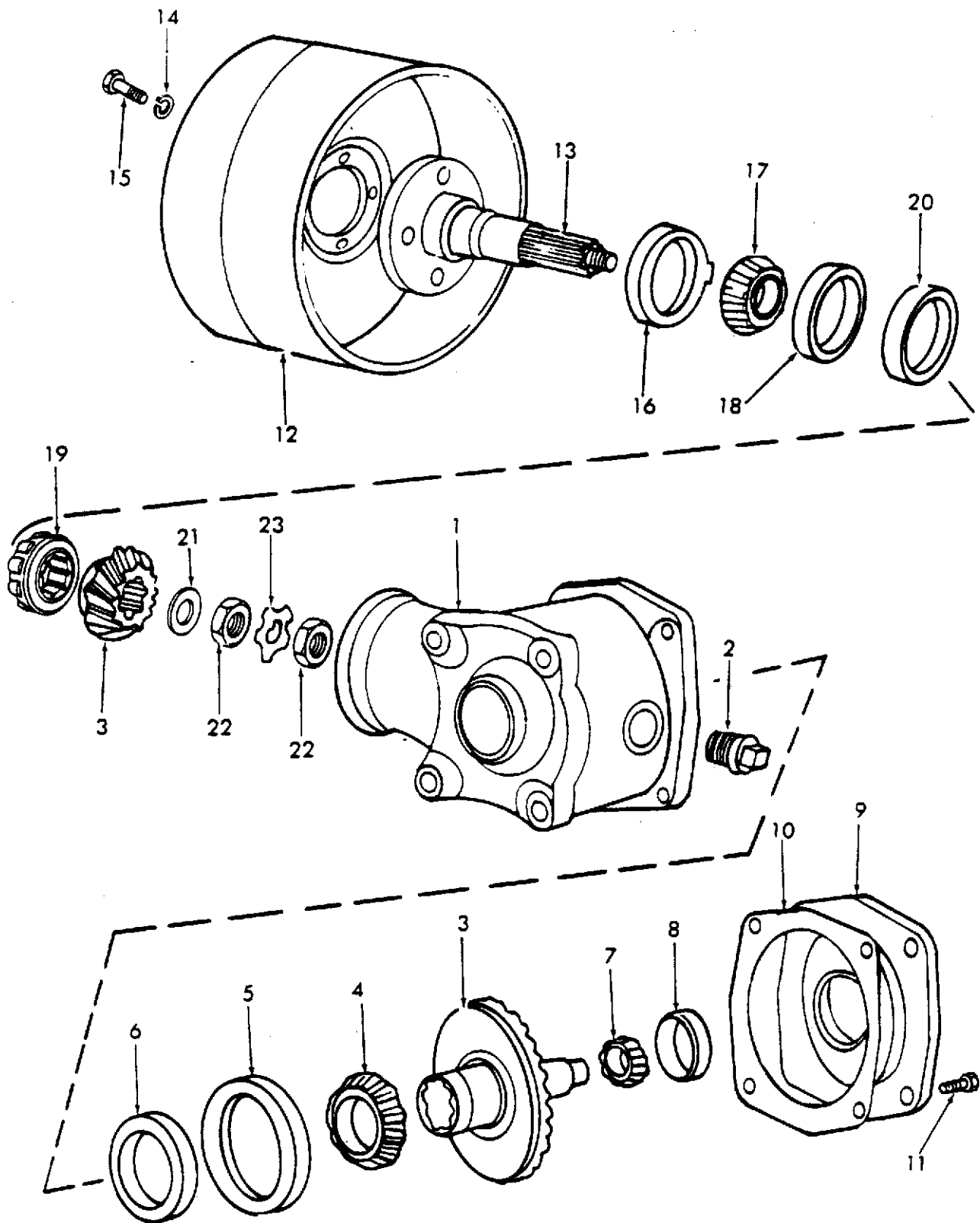
Fig. 33 Pulley Assy.
