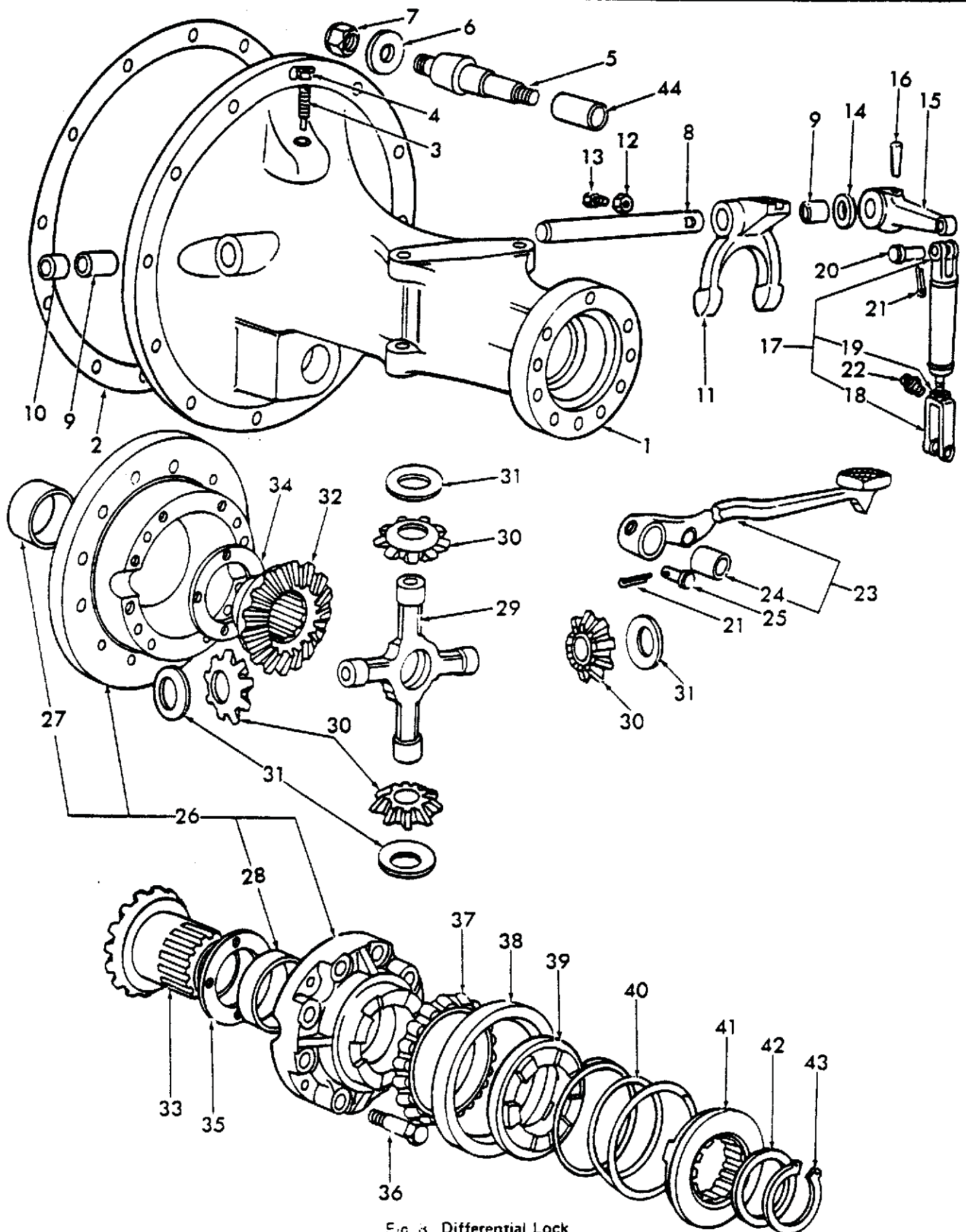
Fig. 3 Differential Lock
