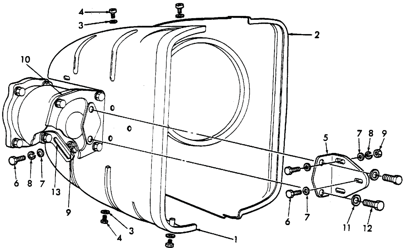
Fig. 34 Pulley Guard
