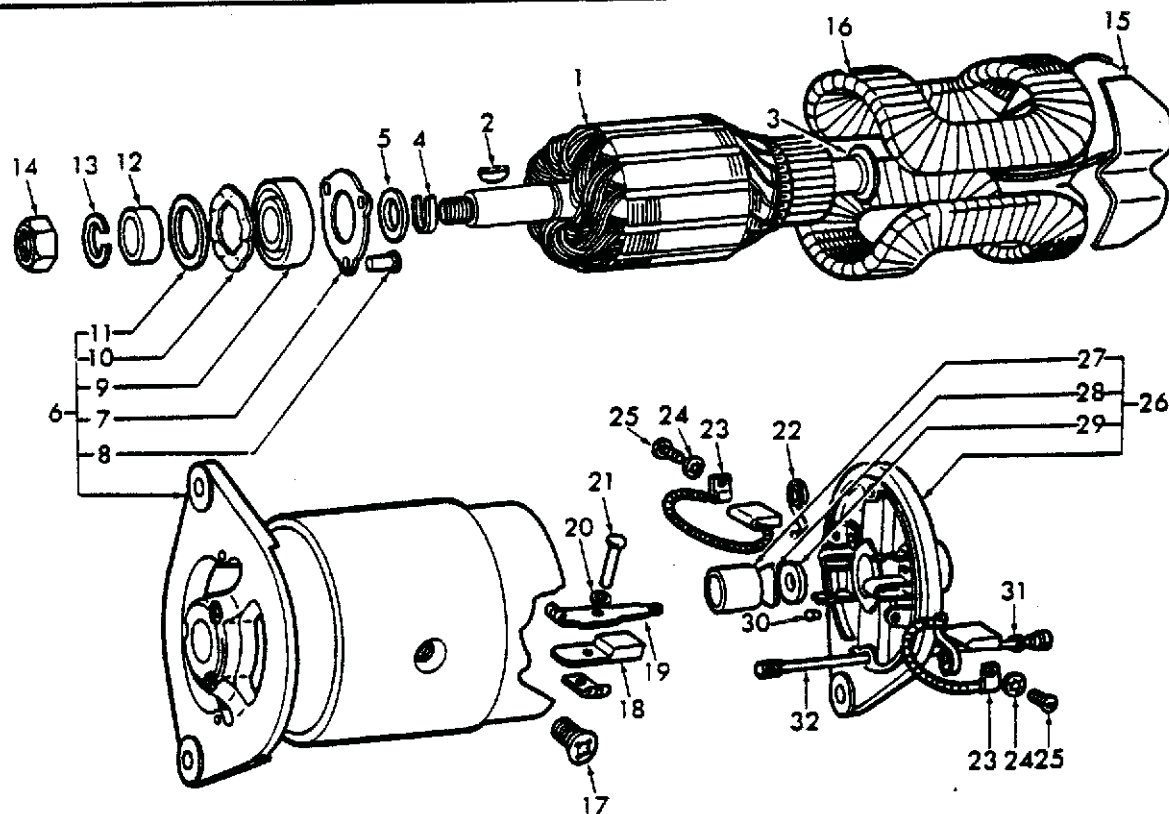
GENERATOR (11-62/64)
