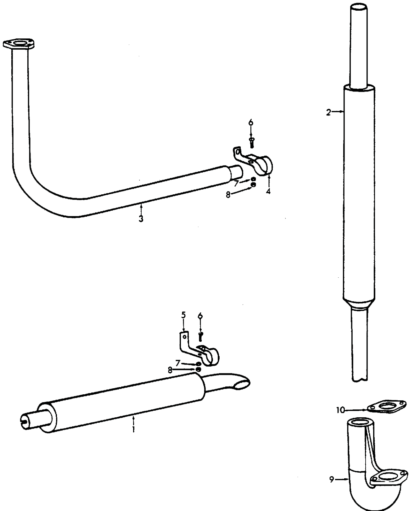
Fig. 26 Mufflers & Related Parts
