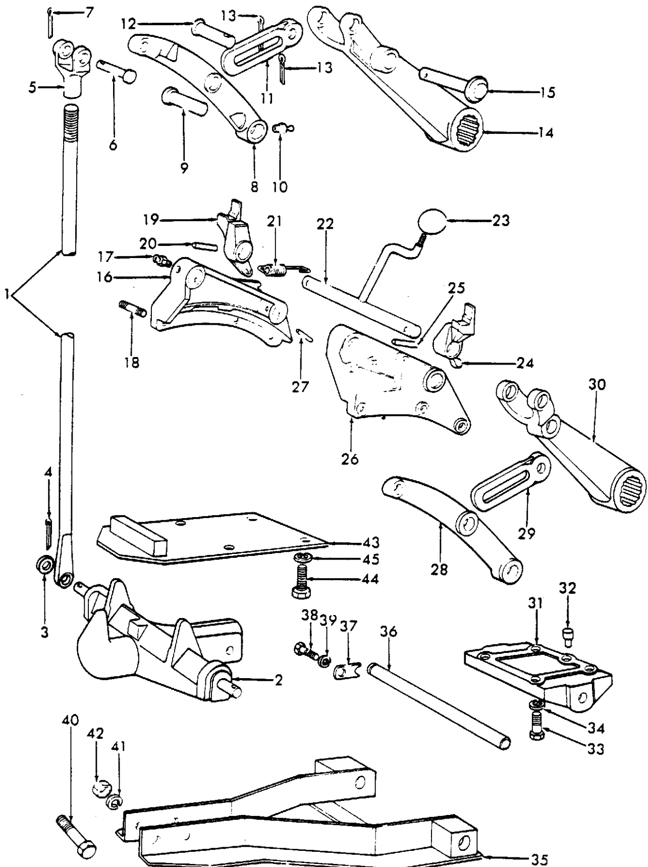
Fig. 18 Automatic Pick-Up Hitch
