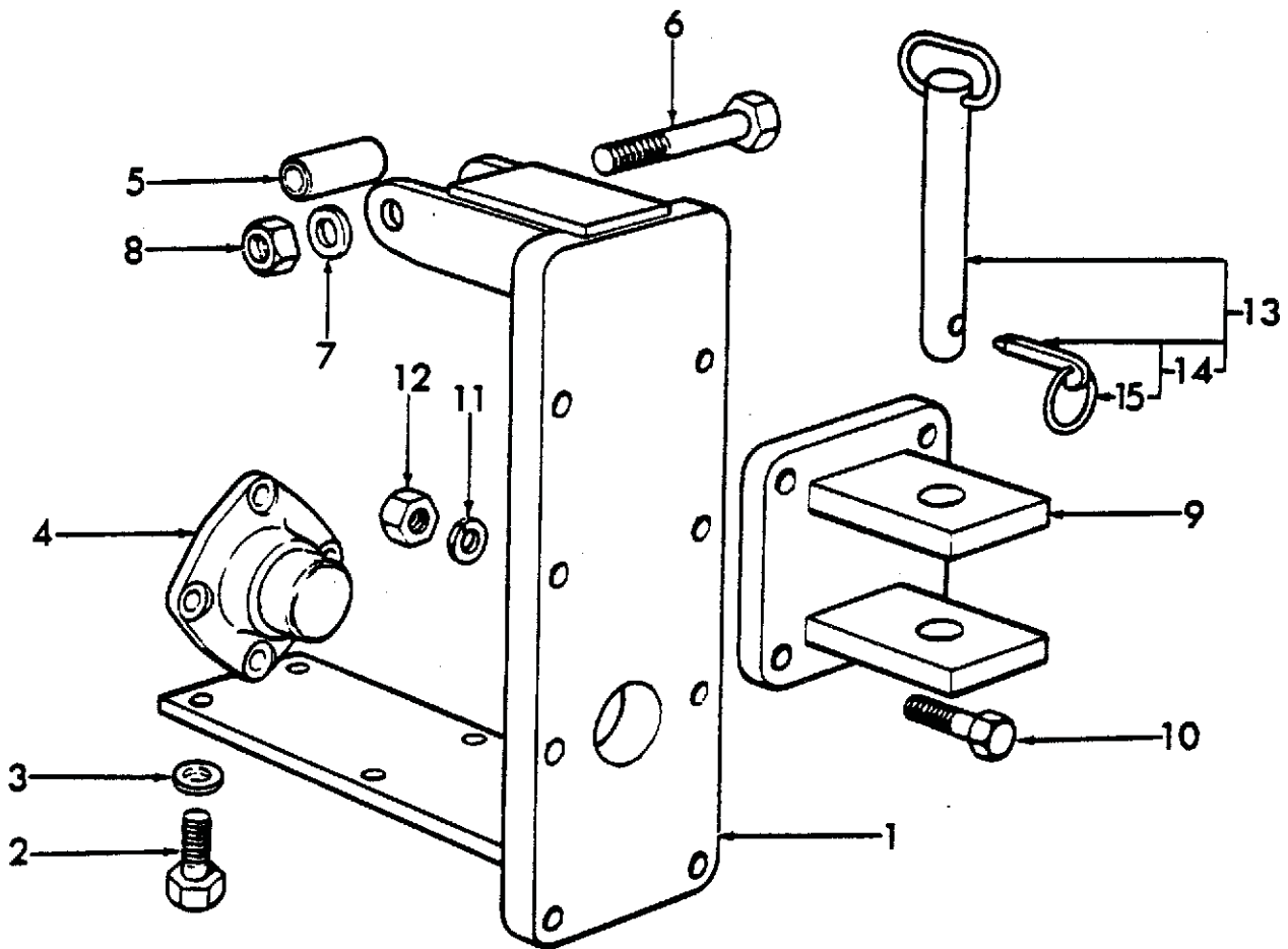
Fig. 57 Drawbar Bracket & Towing Hitch Assy.
