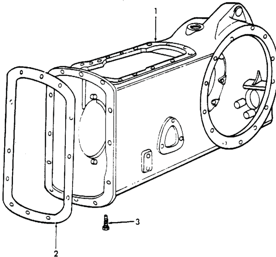
Fig. 9 Differential Housing
