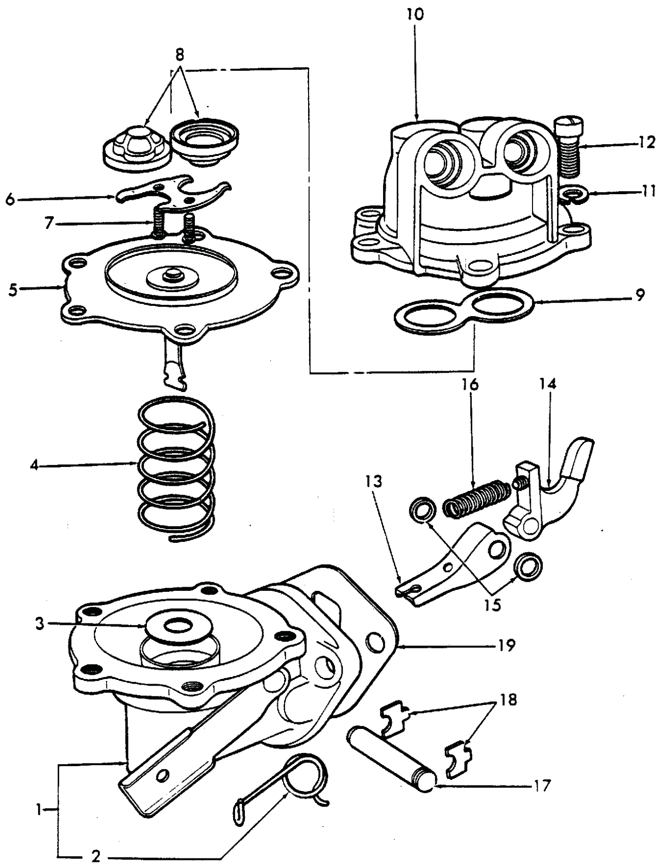
Fig. 45 Fuel Pump Assy.
