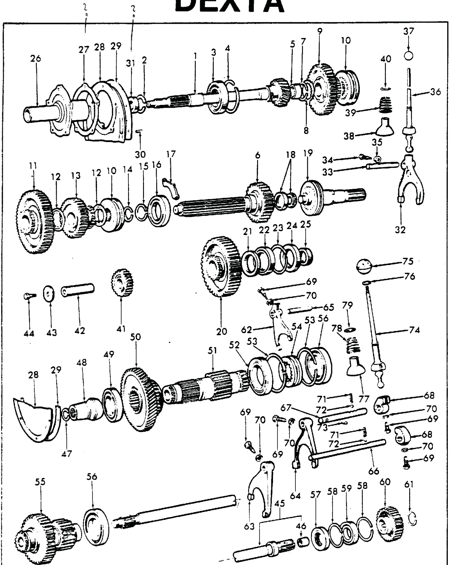
Fig. 26 Front Transmission Interior
